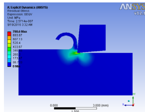
Figure 3.3 Residual Stress 5°
