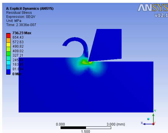
Figure 3.9 Residual Stress 15°
