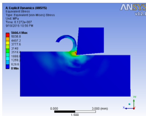
Figure 3.1 Von-mises Stress 5°
